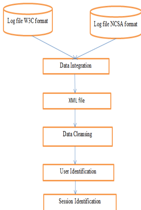
Figure 2.1 Log file Preprocessing
